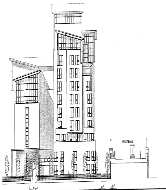
EAST ELEVATION (RIVER FRONTAGE)
